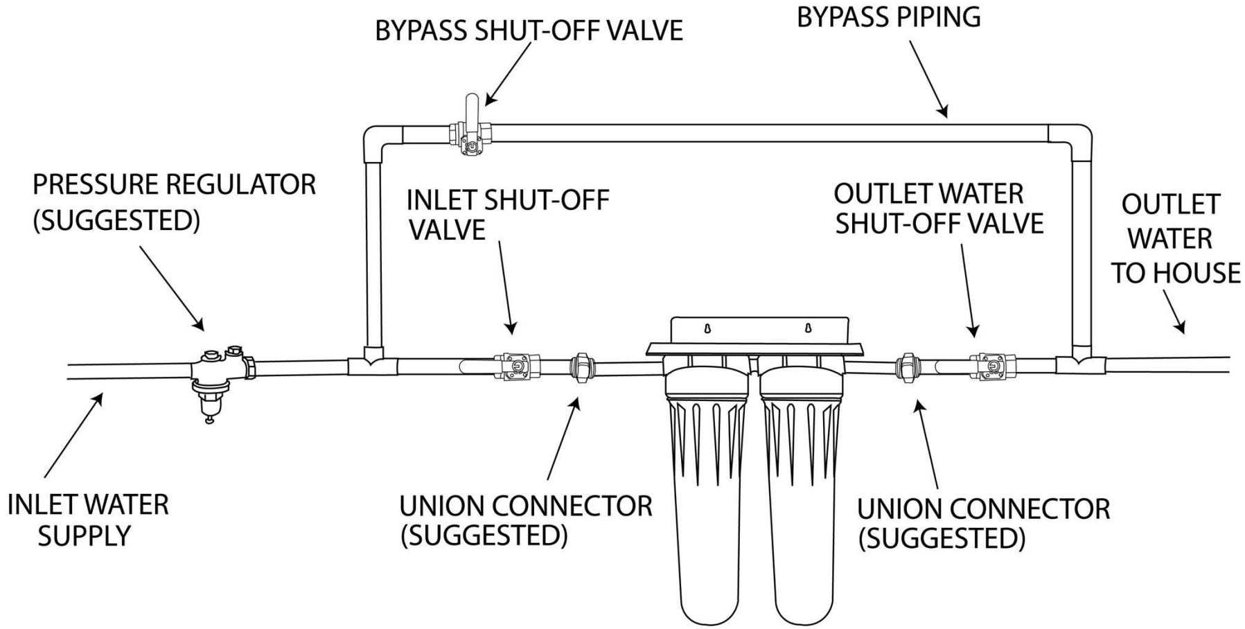
Diagram shows components and parts that are not included with the filter system.
