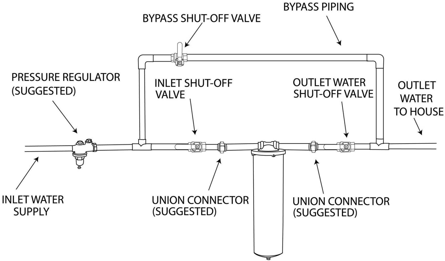
Diagram shows components and parts that are not included with the filter system.
